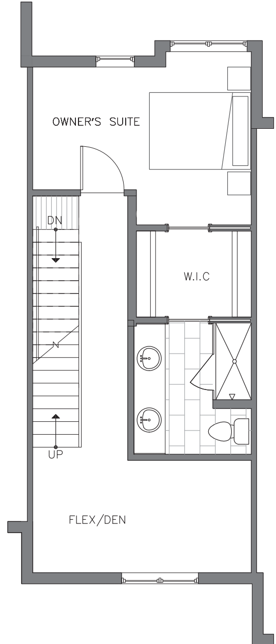
FOURTH FLOOR
